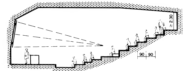
⑤ More steeply raked lecture theatre
